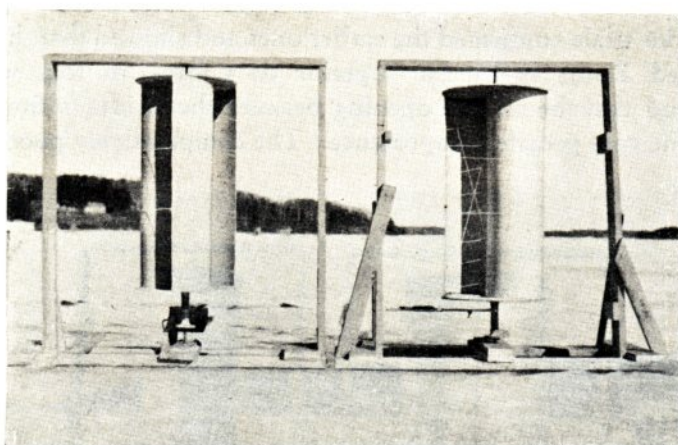
Fig. 8 a. A two winged and a three winged Rotor on the testing stand.
