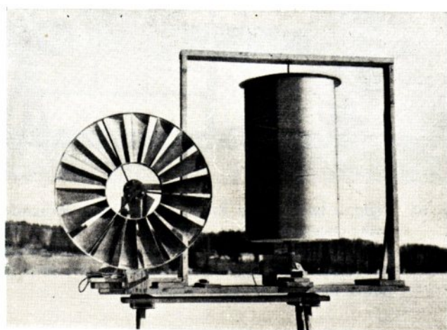
Fig. 11. A Windmill and a Wing-Rotor on the testing stand. See also Fig. 20 b.
